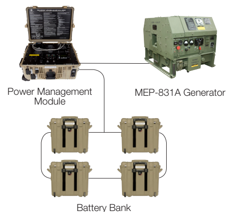
Figure 2 -Example of Hybrid System for Initial Entry Operations
