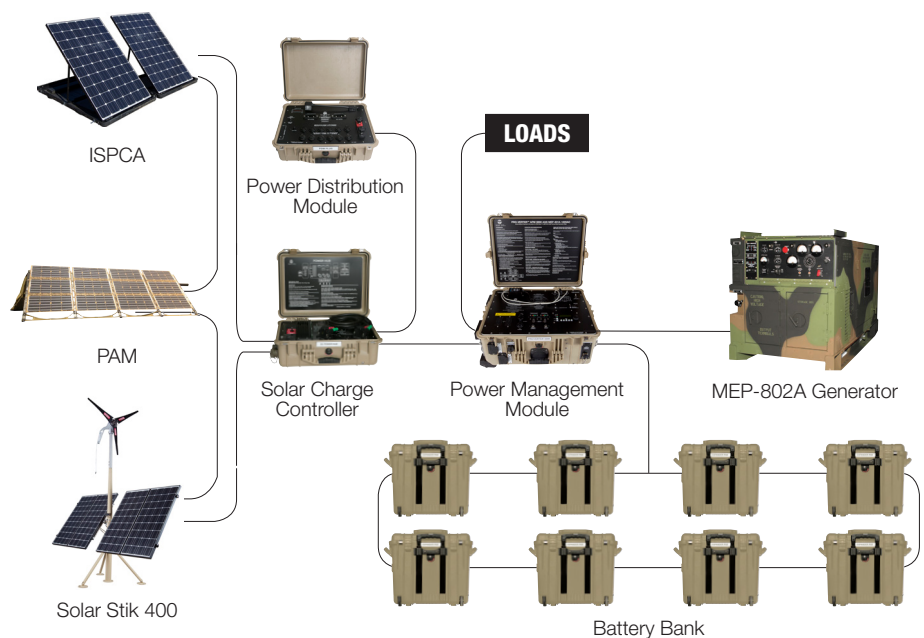
Figure 4 -Hybrid System depicting multiple power sources
