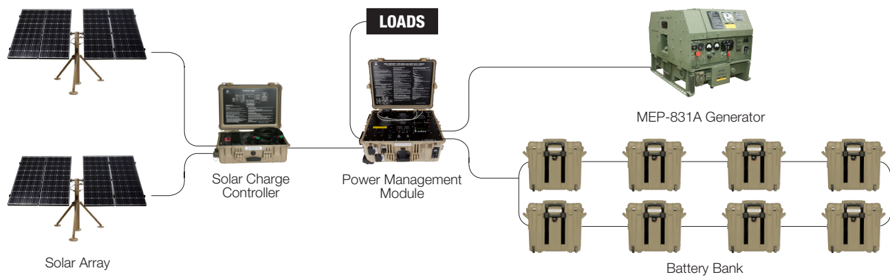
Figure 3 -Example of Hybrid System for Follow-on Operations
