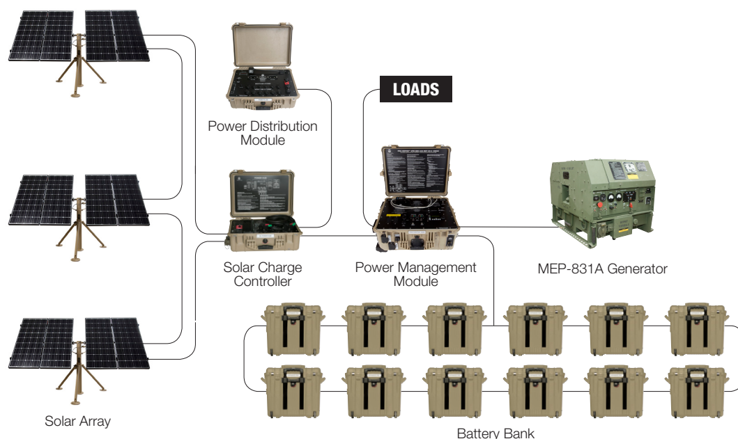
Figure 1 -E2E Deployed Hybrid Power System
